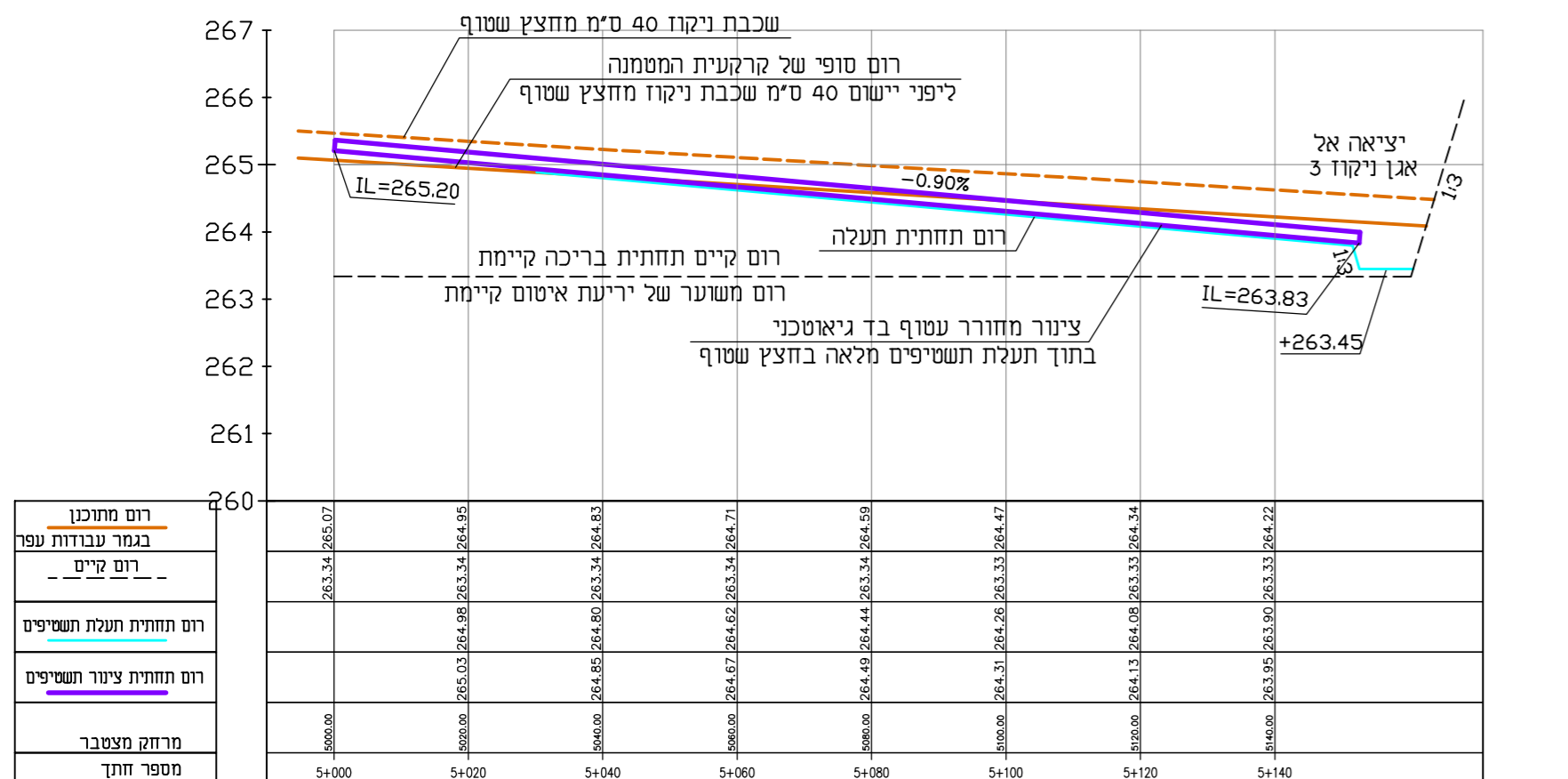
Scale 1:500/50 ROAD NAME tala tasht 5 [tala tasht 5]
