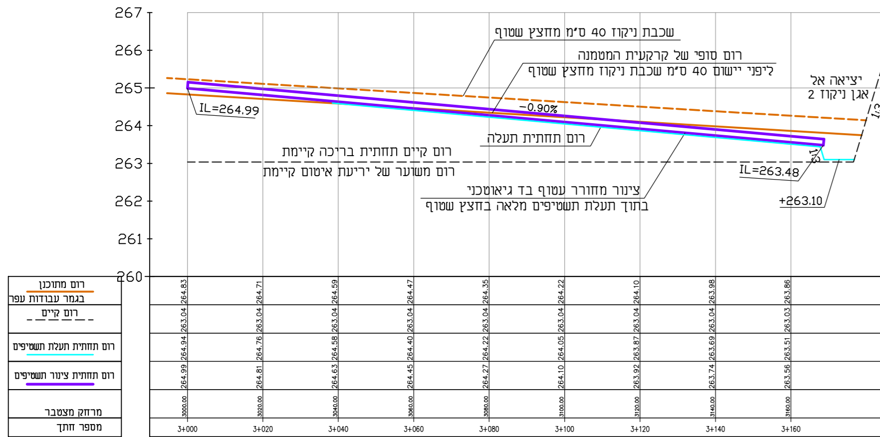
Scale 1:500/50 ROAD NAME tala tasht 3 [tala tasht 3]
