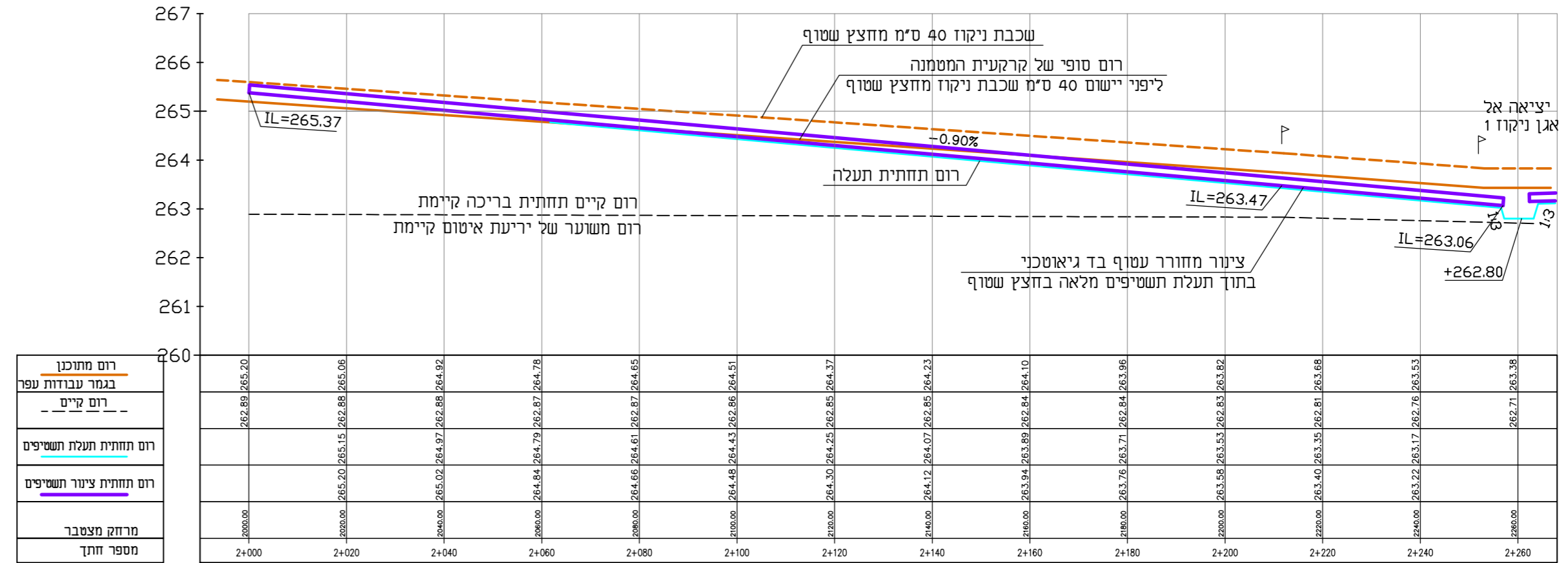
Scale 1:500/50 ROAD NAME tala tasht 2 [tala tasht 2]
